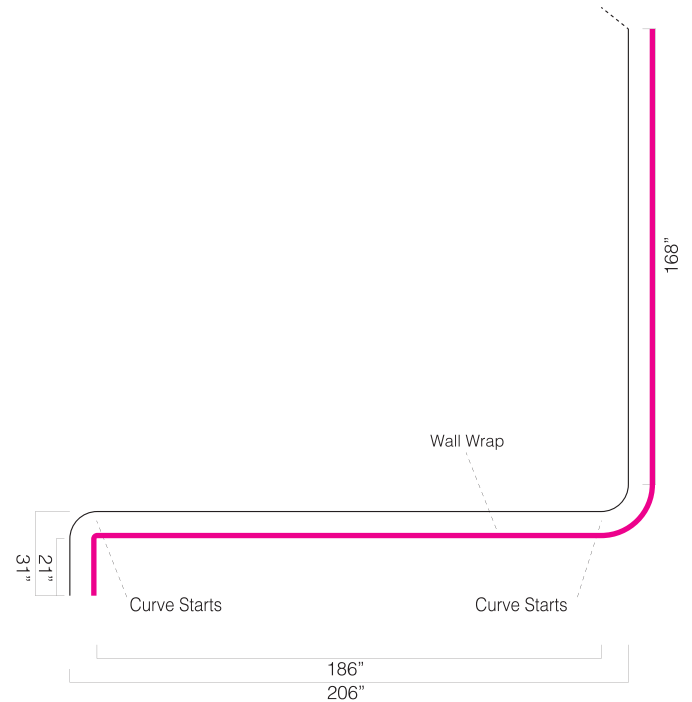
Overhead View Flattened line length 406 1/2"
